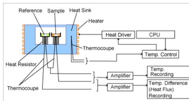
Figure 3: DSC apparatus
