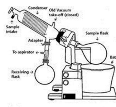
Figure 2: Rotavapour apparatus
