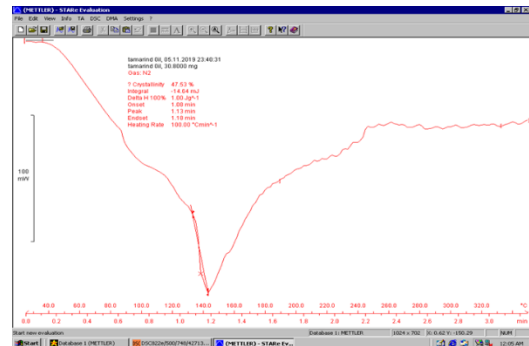
Figure 8: Vaporization point of oil
