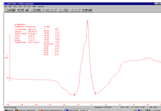
Figure 9: Crystallization point of oil
