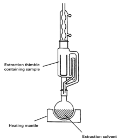
Figure 1: Soxhlet extraction apparatus
